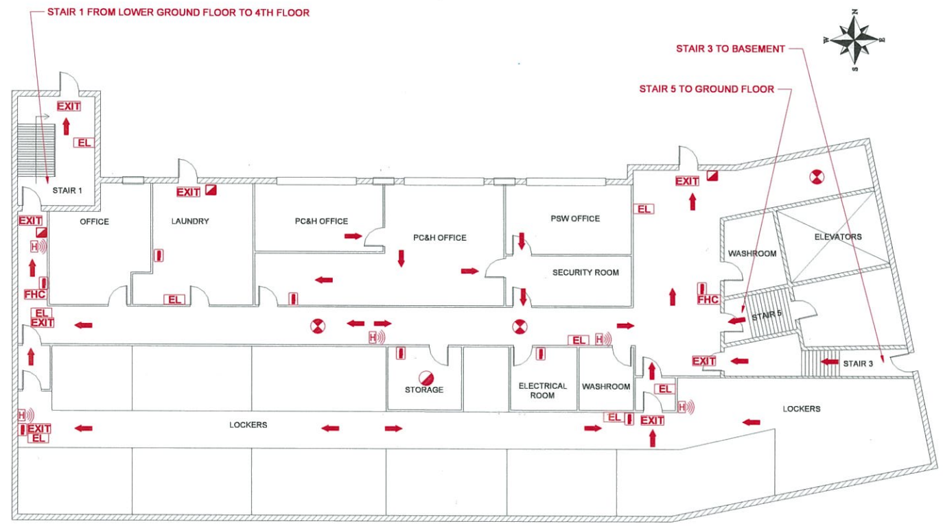
4 Lower Ground Floor Plan Scale: N/A
