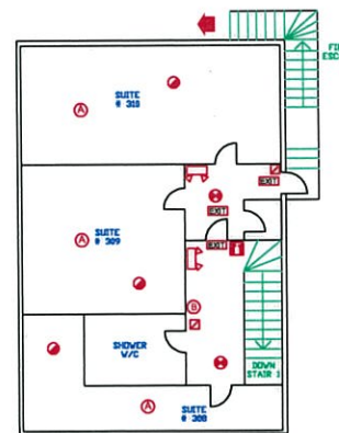
THIRD FLOOR
